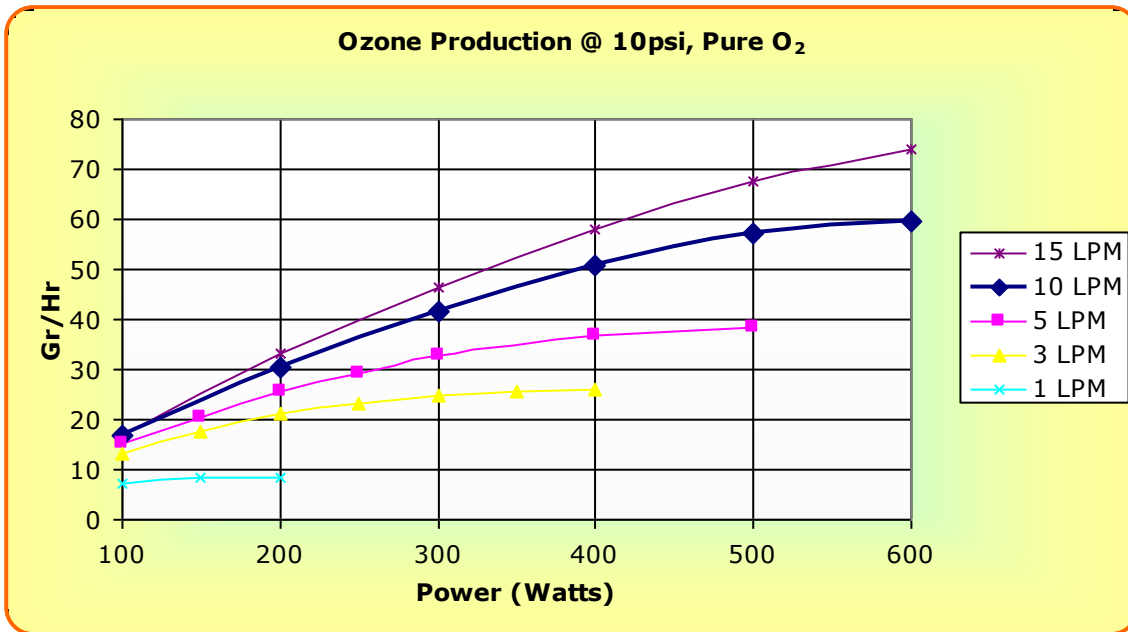
Grams / Hour vs. Power Consumption
